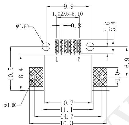
P.C.B. Layout (TOP VIEW) t=1
